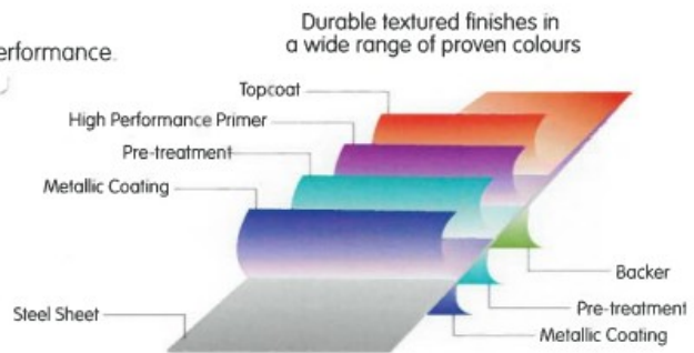
Figure 1. Prepaint system specification
